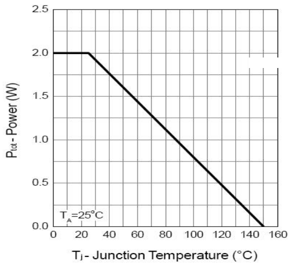
Power Dissipation
